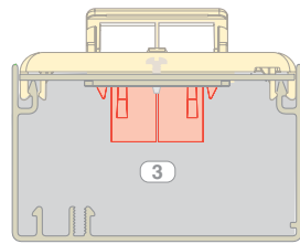
Cable fill #3: Communication pole using vertical sloped snap-on communication faceplate.
